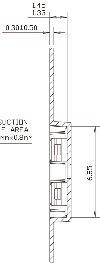
SECTION Y-Y
