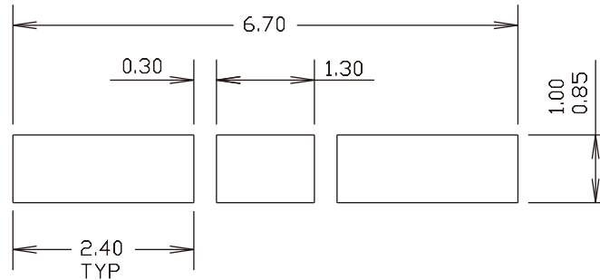
RECOMMENDED P.C.B. PAD LAYOUT
