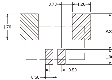
RECOMMENDED P.C.B. LAYOUT (TOP VIEW) TOLERANCE ±0.05mm
