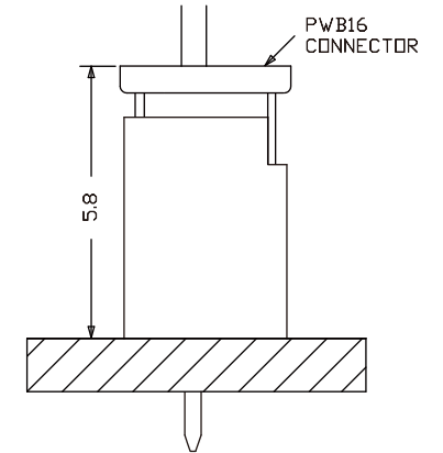
MATED CONNECTOR FIGURE
