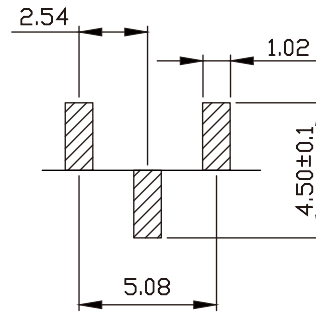
RECOMMENDED P.C.B. LAYOUT (TOP VIEW) TOLERANCE ±0.05mm
