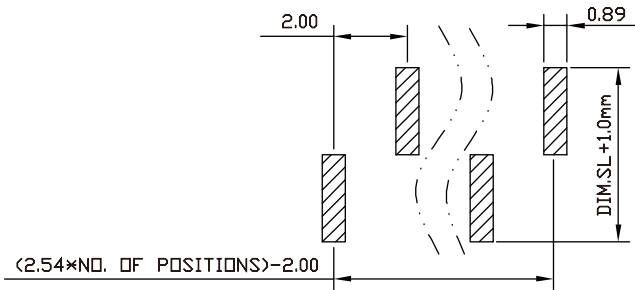
(TYPE T) RECOMMENDED P.C.B. LAYOUT
