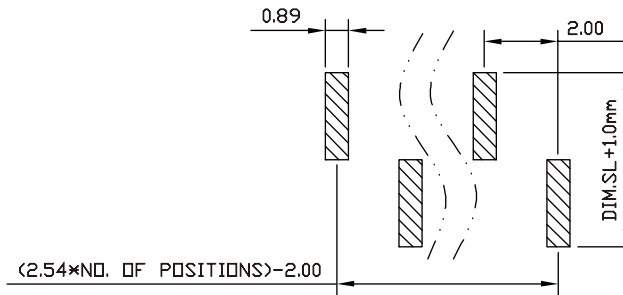
(TYPE D) RECOMMENDED P.C.B. LAYOUT
