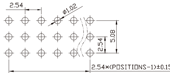
RECOMMENDED P.C.B. LAYOUT (TOP VIEW) TOLERANCE ± 0.05mm
